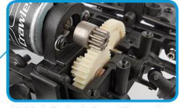
13.98:1 Ratio 3-Gear Transmission with Integrated Motor Mount
