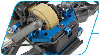
Gear Differential and Anti-Roll Bars
